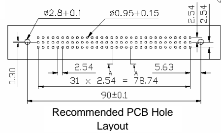
All dimensions in mm
