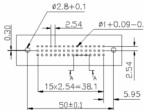
Recommended PCB Hole Layout Component Side
