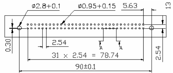
Recommended PCB Hole Layout
