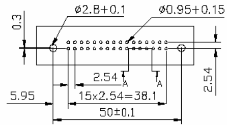
Recommended PCB Hole Layout Component Side
